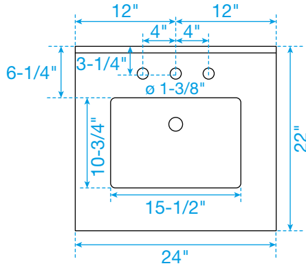
TOP VIEW OF VANITY CABINET
